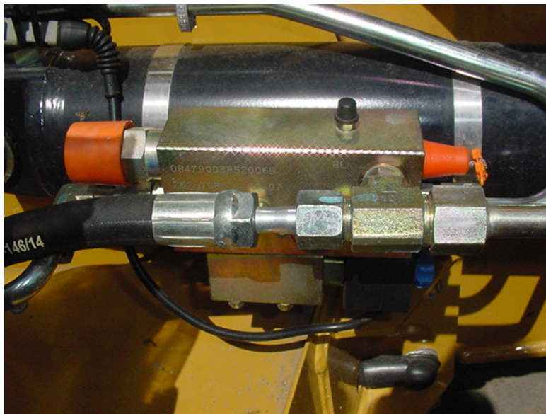
Fig 3 - Typical Lowering Control Valve Installation.
